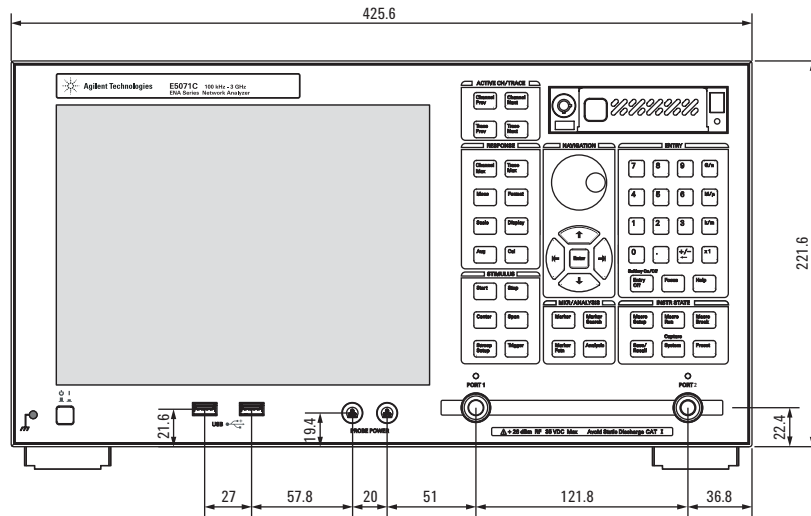
Figure 2. Dimensions (front view, E5071C with option 230/235/240/245/280/285, in millimeters)
