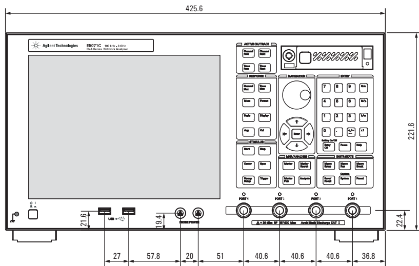
Figure 3. Dimensions (front view, E5071C with option 430/435/440/445/480/485, in millimeters)
